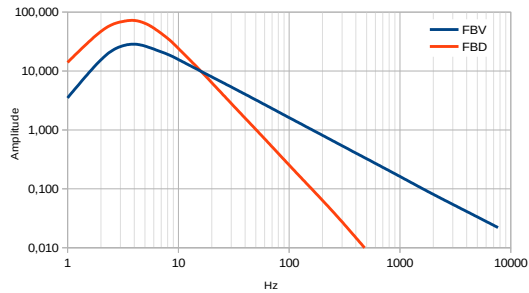
Figure 6: Amplitude response of integrators
