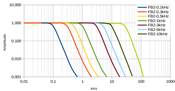
Figure 4: Amplitude response of low pass filters
