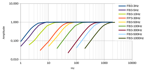
Figure 5: Amplitude response of high pass filters
