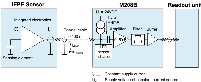
Figure 2: IEPE principle
