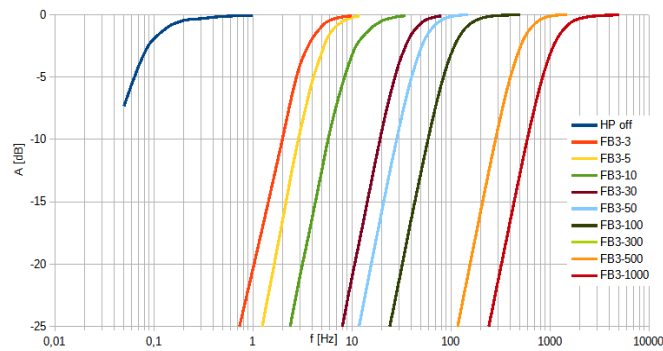
Amplitude Response
